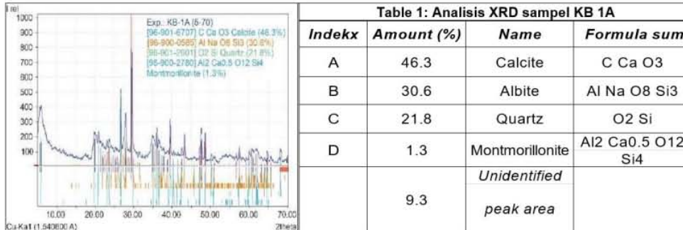
Figure 3: The diffractogram of soil sample KB 1A
